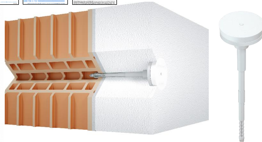
ECO-DRIVE S 8 - Screwed-in fastener with metal pin and telescopic support collar
