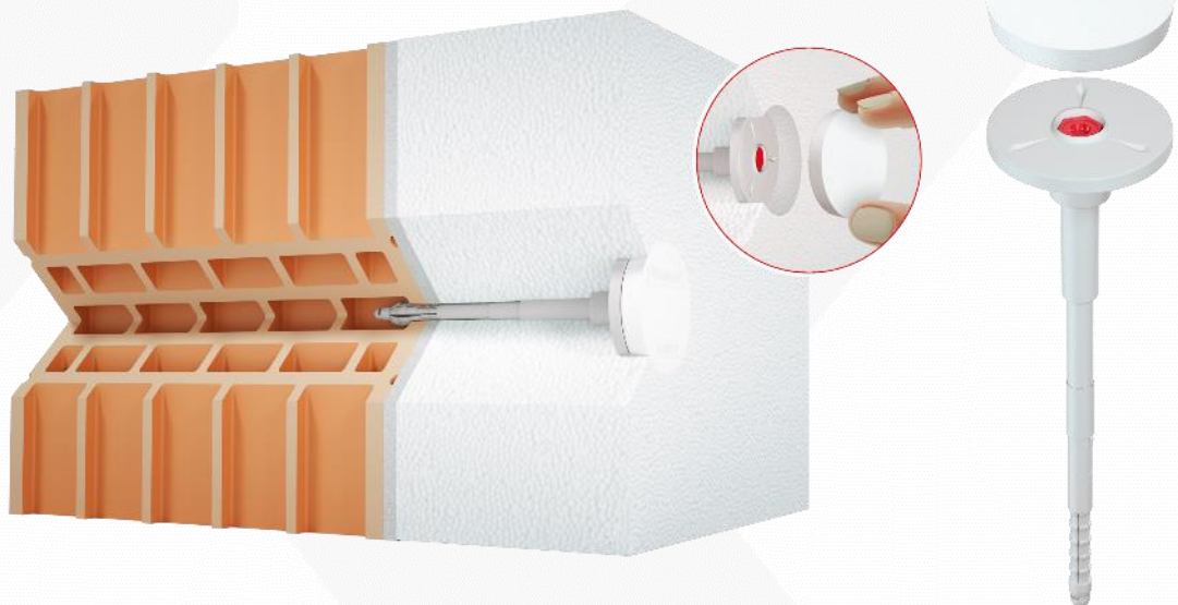
ECO-DRIVE 8 - Screwed-in fastener with metal pin and telescopic support collar
