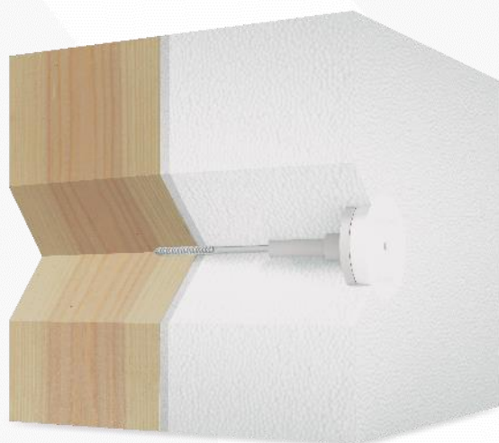
ECO-DRIVE 8 - Screwed-in fastener with metal pin and telescopic support collar
